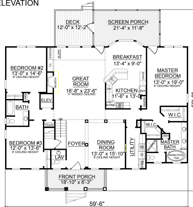
FIRST FLOOR PLAN Plan No.
